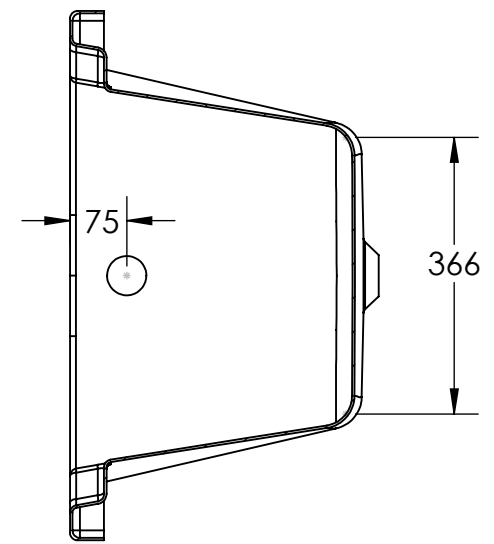
SECTION BL-BL SCALE 1 : 10
